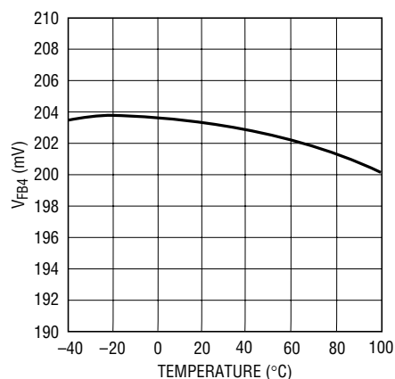
FB4 Voltage
