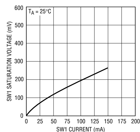
SW1 Saturation Voltage
