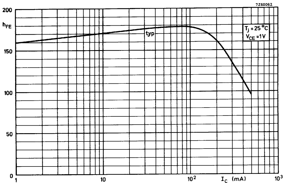
Fig. 2 DC current gain.
