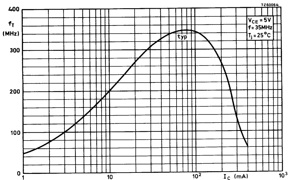
Fig. 7 Typical values transition frequency.
