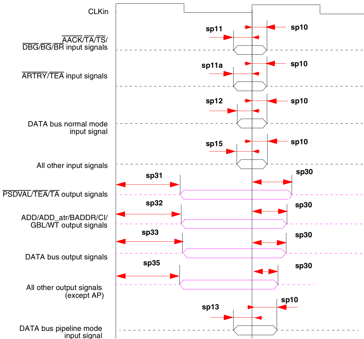
Figure 9. Bus Signals
