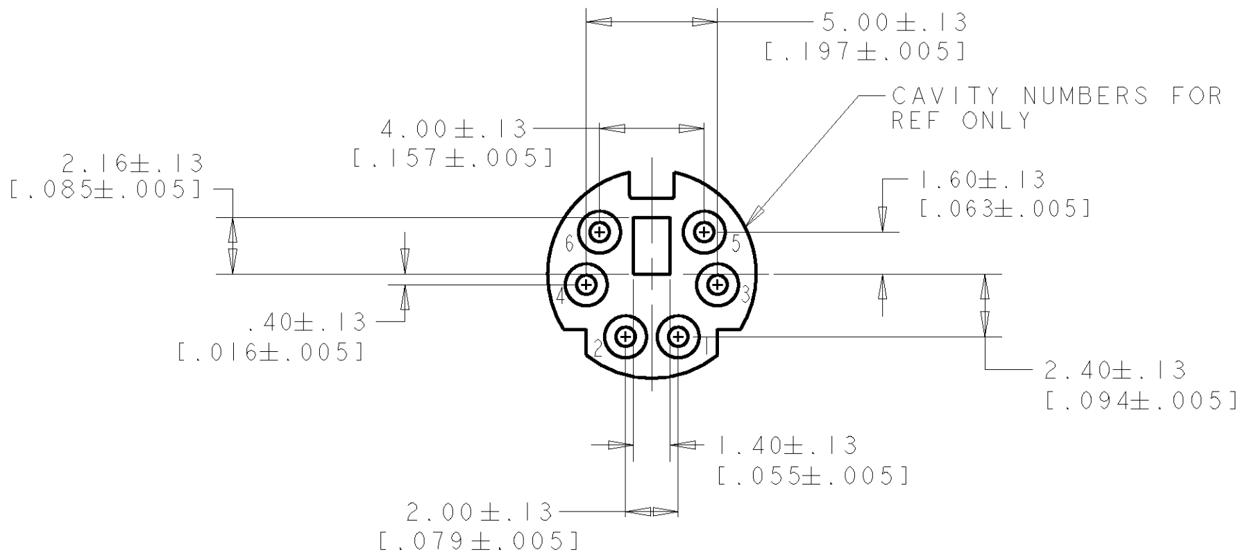
DETAIL D 6 PIN FACE
