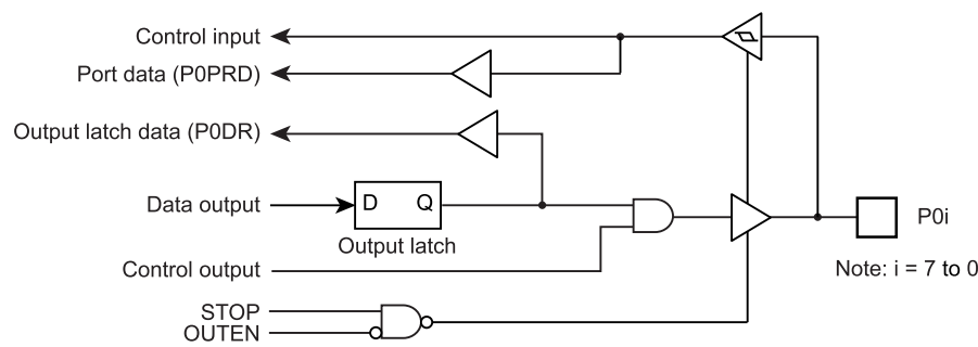
Figure 7-2 Port P0
