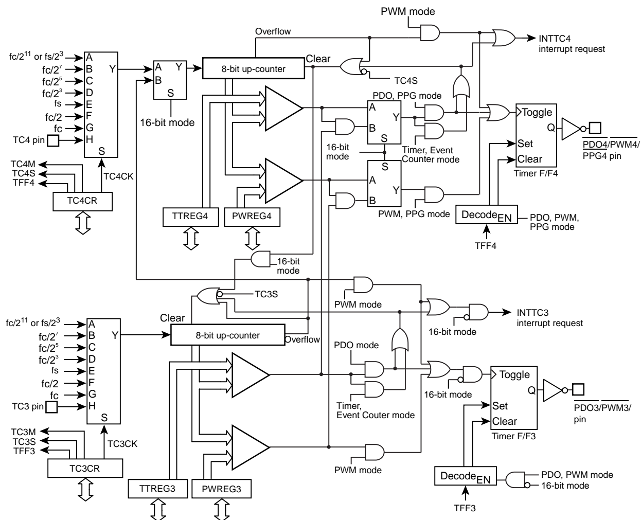
Figure 9-1 8-Bit TimerCounter 3, 4
