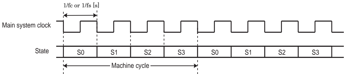
Figure 2-5 Machine Cycle
