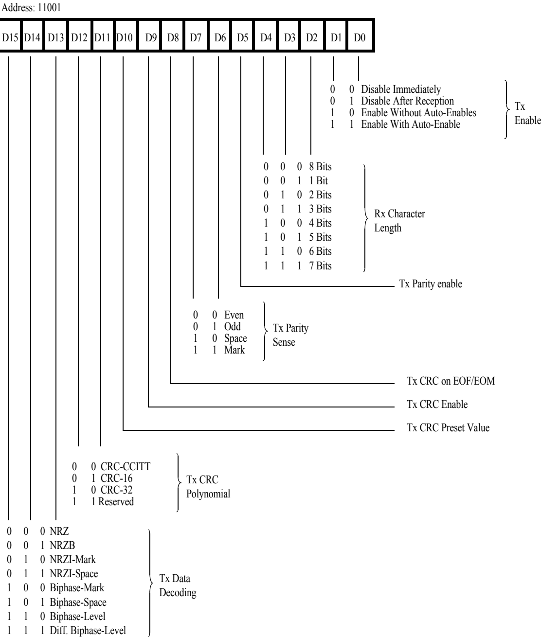
Figure 67. Transmit Mode Register
