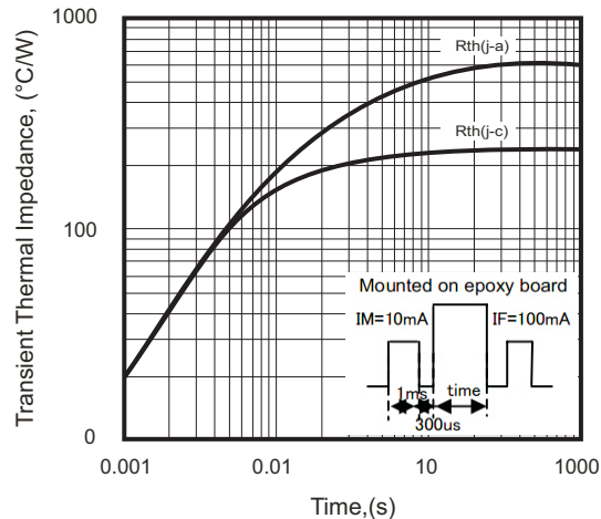
Fig.5 - Rth-t Characteristics
