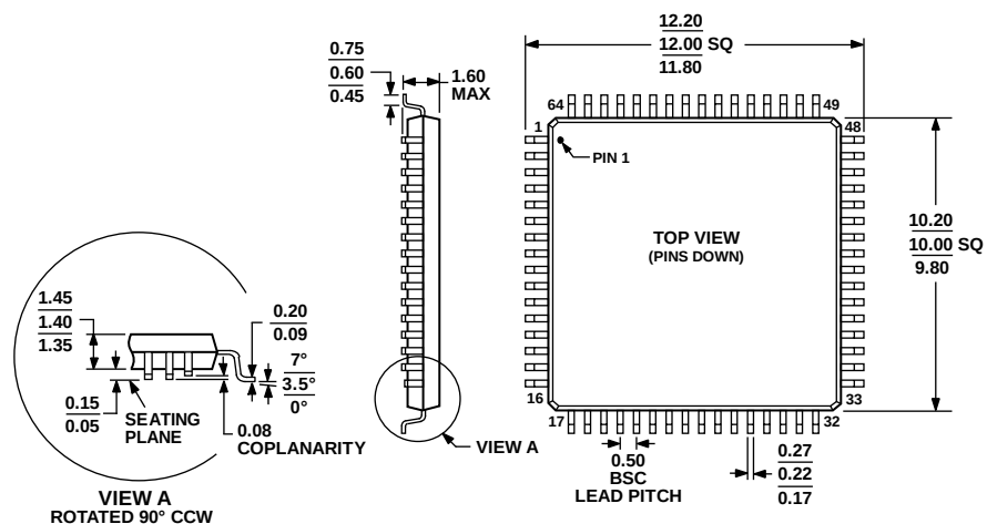
Figure 63. 64-Lead Low Profile Quad Flat Package [LQFP] 10 mm x 10 mm Body (ST-64-2)
