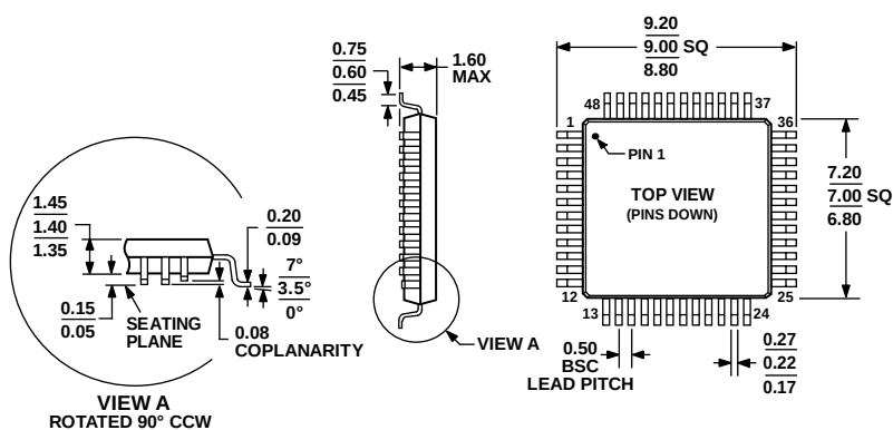
Figure 64. 48-Lead Low Profile Quad Flat Package [LQFP] 7 mm x 7 mm Body (ST-48)
