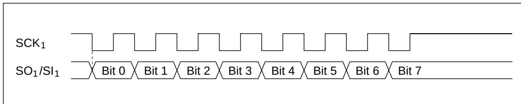
Figure 10-2-2 Transfer Format
