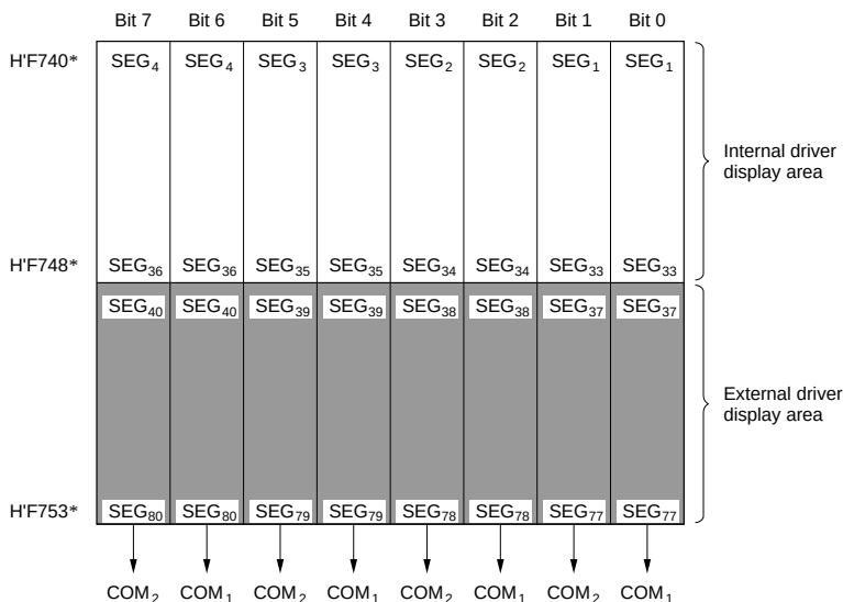
Figure 12-7 LCD RAM Map 1: External Segment Expansion (1/2 Duty)
