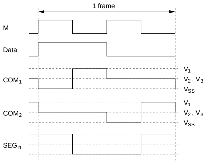
Figure 12-11 (c) Waveforms at 1/2 Duty
