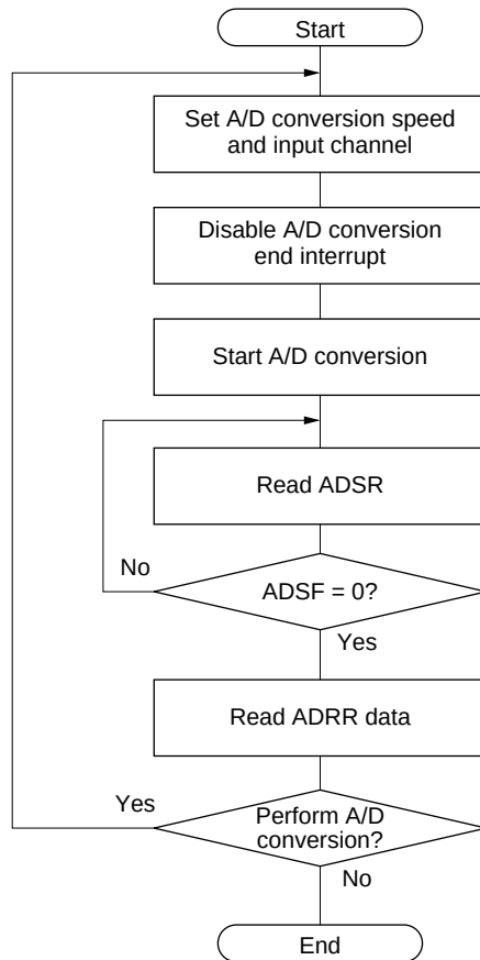
Figure 11-4 Flow Chart of Procedure for Using A/D Converter (1) (Polling by Software)
