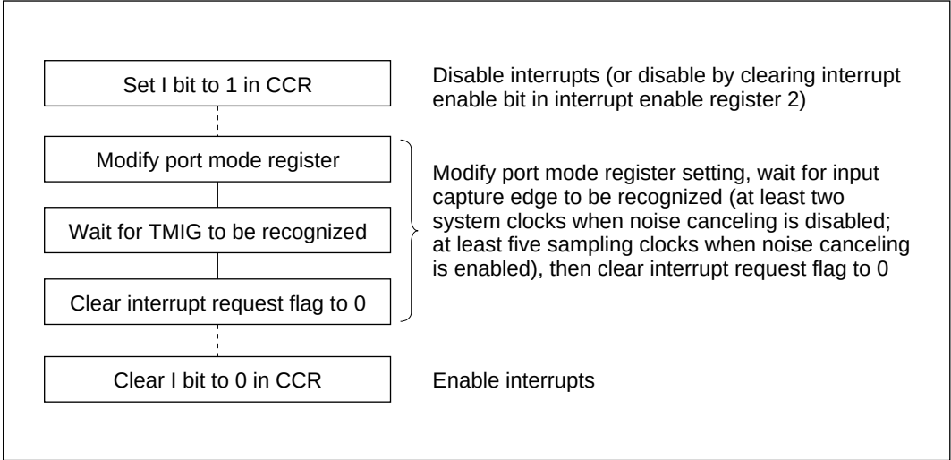
Figure 9-4-8 Procedure for Modifying Port Mode Register and Clearing Interrupt Request Flag
