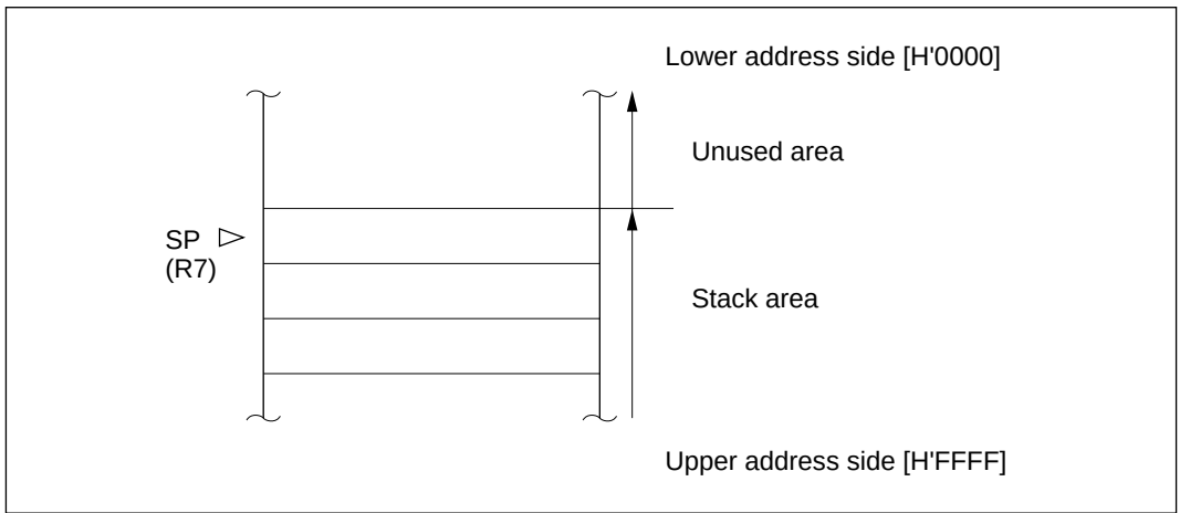
Figure 2-2 Stack Pointer
