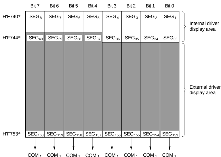
Figure 12-8 LCD RAM Map 2: External Segment Expansion (Static Duty)
