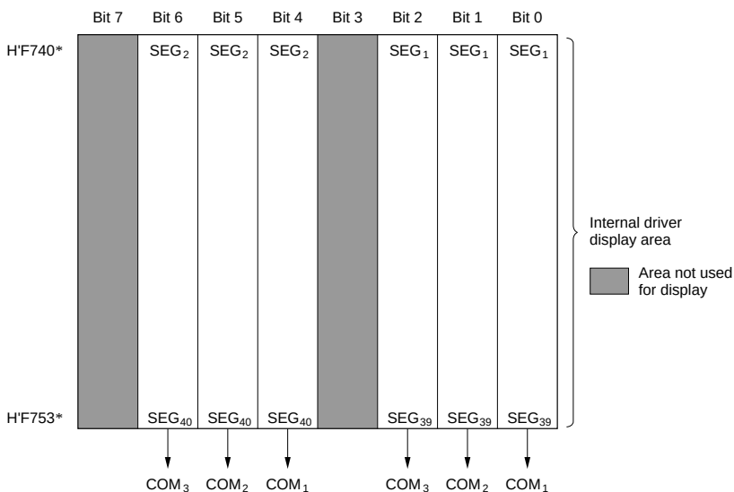
Figure 12-4 LCD RAM Map 2: No External Segment Expansion (1/3 Duty)
