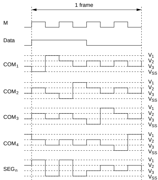
Figure 12-11 (a) Waveforms at 1/4 Duty
