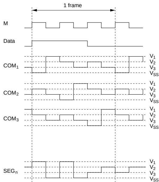
Figure 12-11 (b) Waveforms at 1/3 Duty
