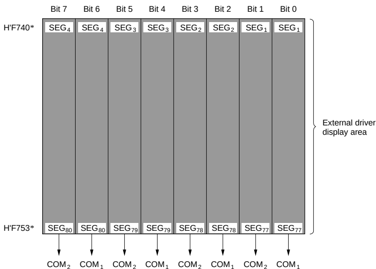
Figure 12-9 LCD RAM Map When All External Segments are Used (Example: SGX = 1, SGS3 to SGS0 = 0000, 1/2 Duty)
