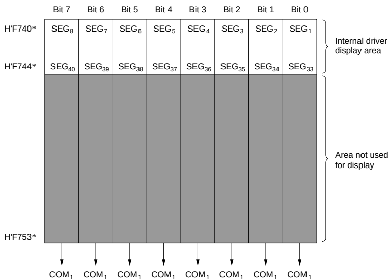
Figure 12-6 LCD RAM Map 4: No External Segment Expansion (Static Duty)
