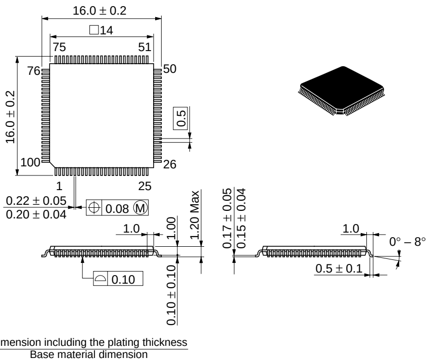
Figure F-3 TFP-100B Package Dimensions
