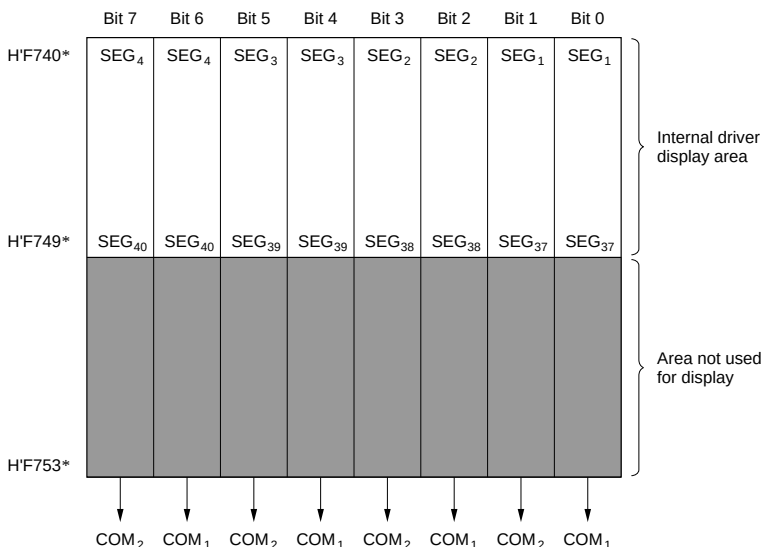
Figure 12-5 LCD RAM Map 3: No External Segment Expansion (1/2 Duty)
