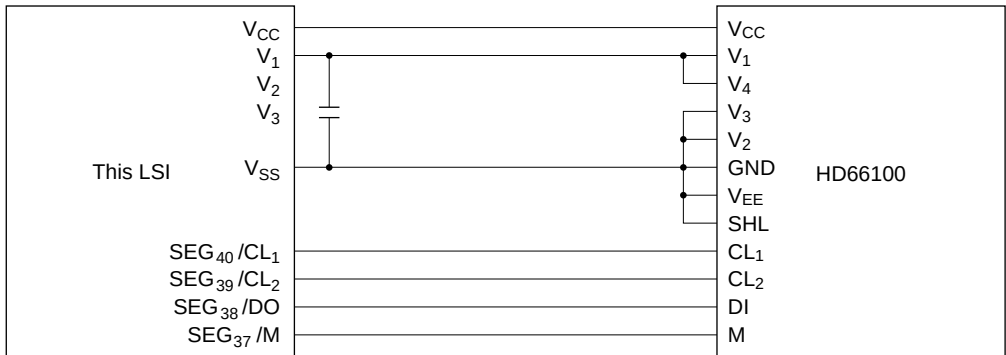
Figure 12-10 Connection to HD66100
