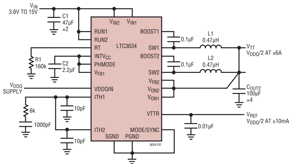
Figure 7. Application Circuit for a 2-Phase, \pm 6\text{A} Single V_{\Pi} Output
