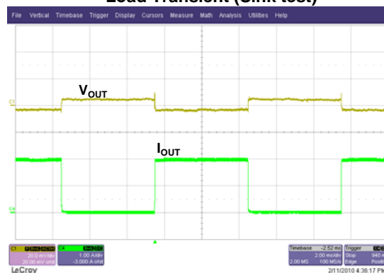
Load Transient (Sink test)
