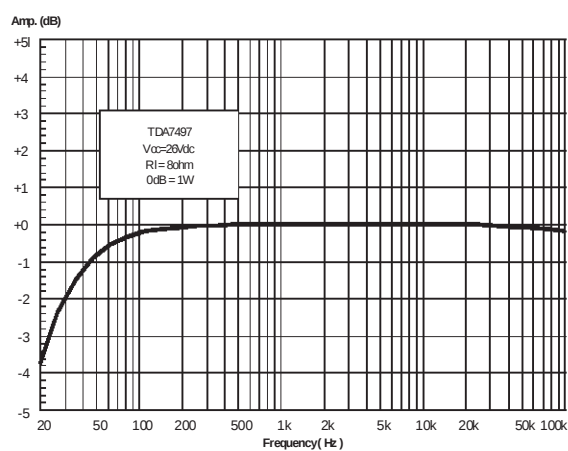
Figure 4. Frequency Response
