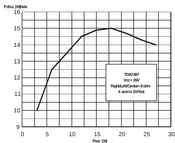
Figure 7. P diss vs Output Power
