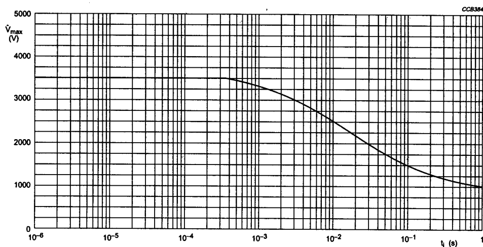
Fig. 30 Pulse on regular basis; maximum permissible peak pulse voltage ( V_{max} ) as a function of pulse duration ( t_i )
