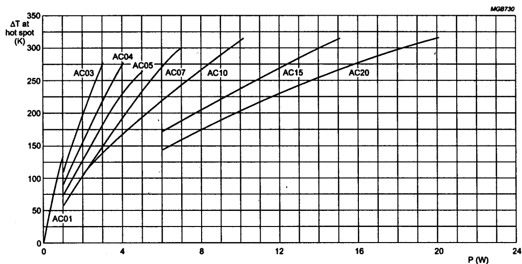
Fig. 3 Hot spot temperature rise ( \Delta T ) as a function of dissipated power.
