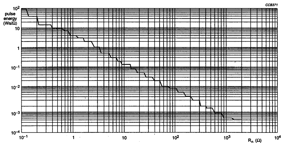
Fig. 13 Pulse capability; Ws as a function of R n
