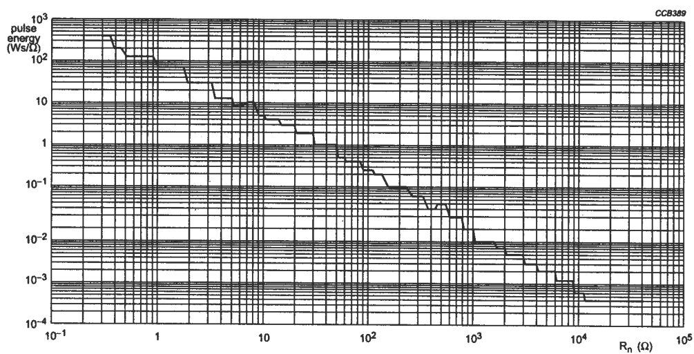
Fig. 34 Pulse capability; W_s as a function of R_n
