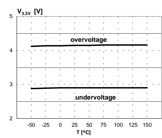
Figure 5. 3.3V fault thresholds
