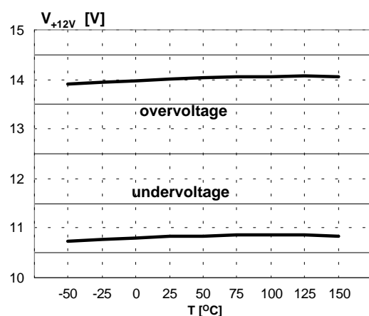
Figure 7. 12V fault thresholds
