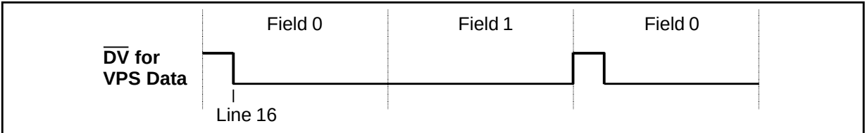
Figure 6 : Data Valid Timing ( \overline{DV} )
