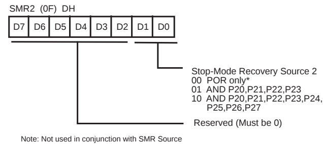
Figure 38. Stop-Mode Recovery Register2
