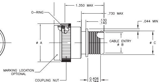
SELF-LOCKING SHIELD BAND TERMINATION SHRINK BOOT ACCOMMODATION ADAPTER
