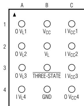
3 x 4 UCSP
