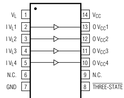
TSSOP-14
