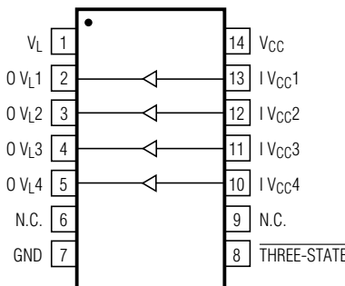
TSSOP-14
