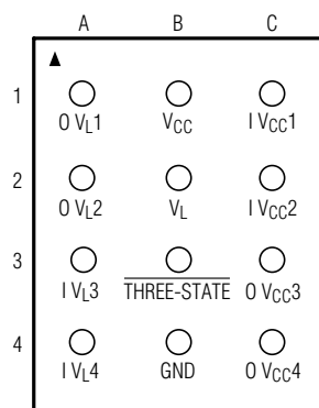
3 x 4 UCSP
