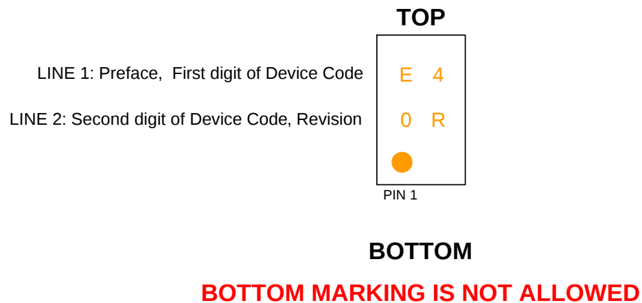
Figure 8.4 EMC1186-1 8-Pin TDFN Package Markings
