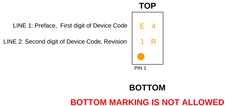
Figure 8.5 EMC1186-2 8-Pin TDFN Package Markings
