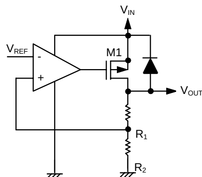
Figure 7 Voltage Regulator
