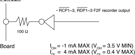
Output Circuit
