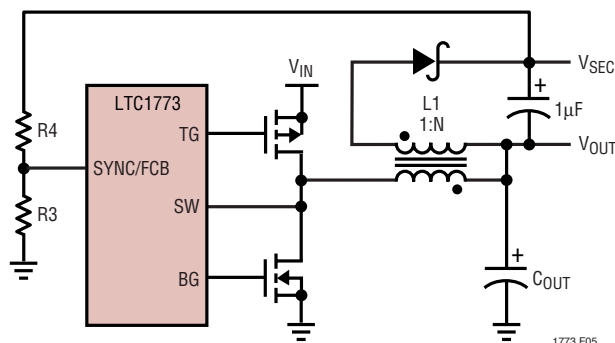
Figure 5. Secondary Output Loop Connection
