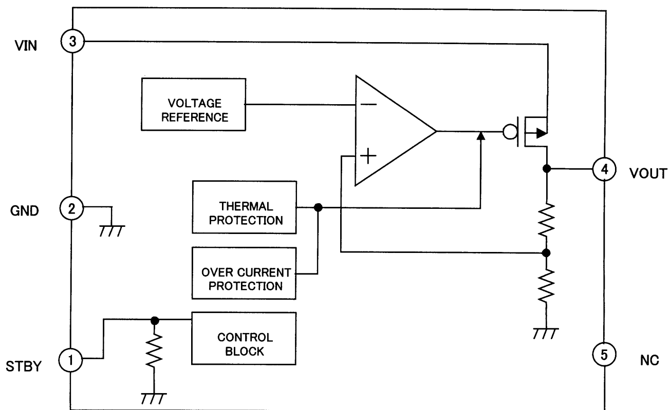
Fig.2 BLOCK DIAGRAM
