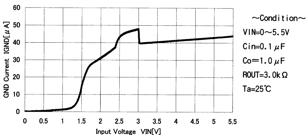
Fig.11 GND Current-Input Voltage
