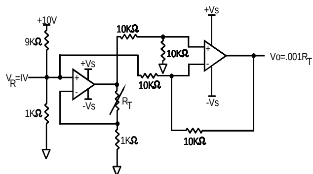
Fig. 2: Linear Output Voltage
