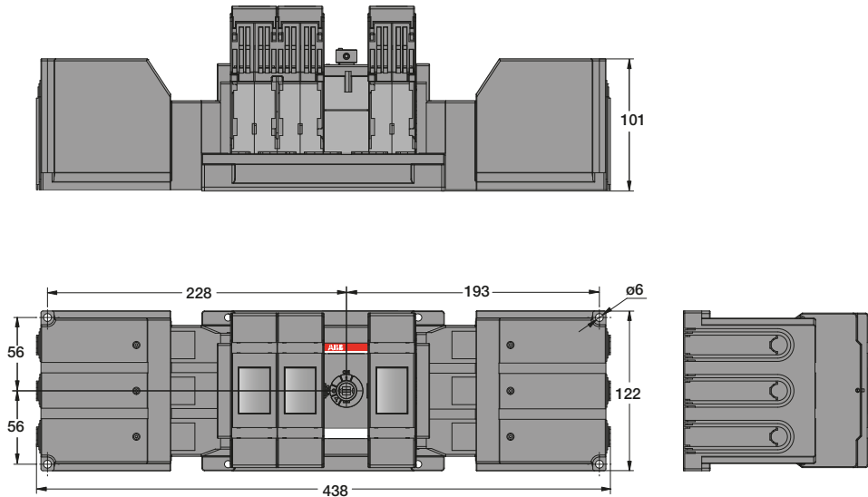
OS125G...160G_21LR + OSS160G T G 3LS
