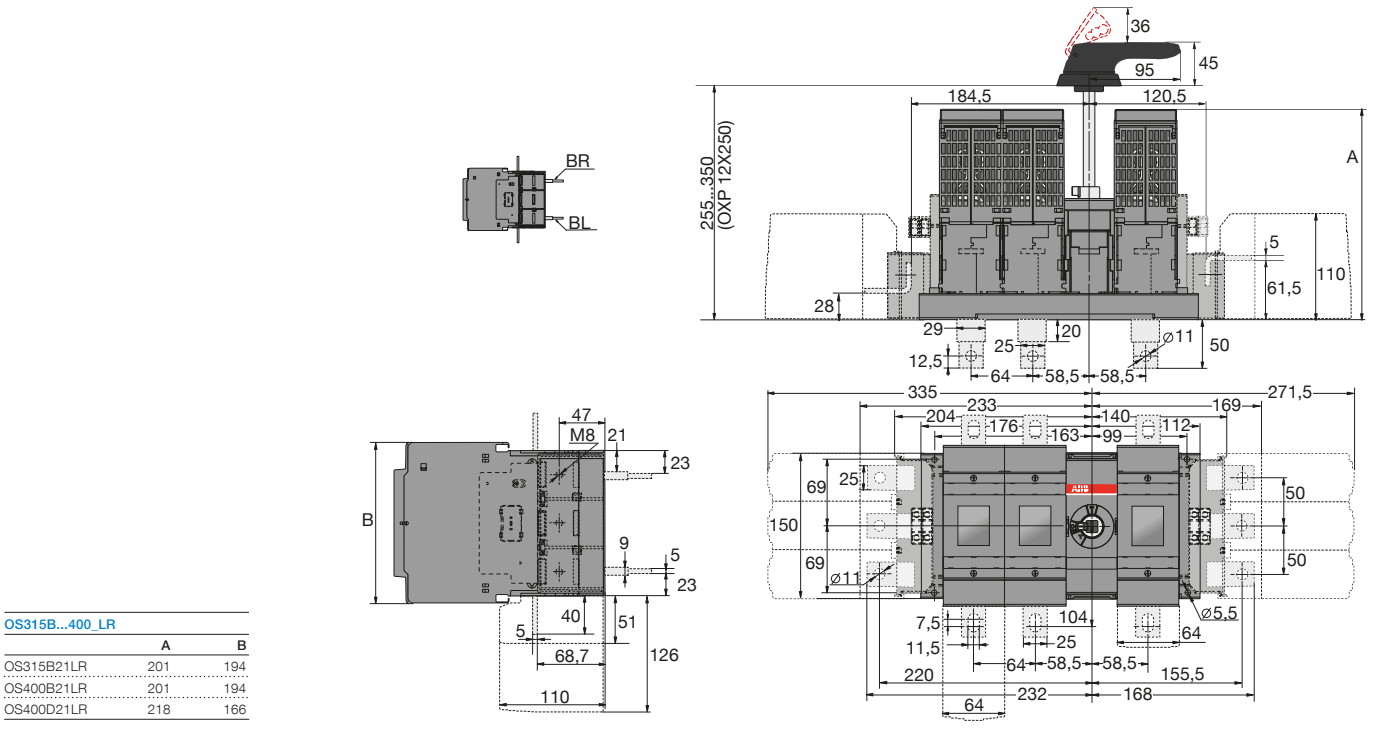
OS315B21_ and OS400_21_ (LR)
