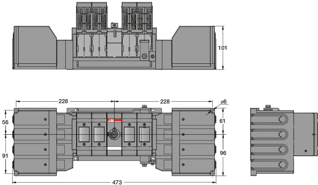
OS125G...160G_22LR + OSS160G T G 4LS
