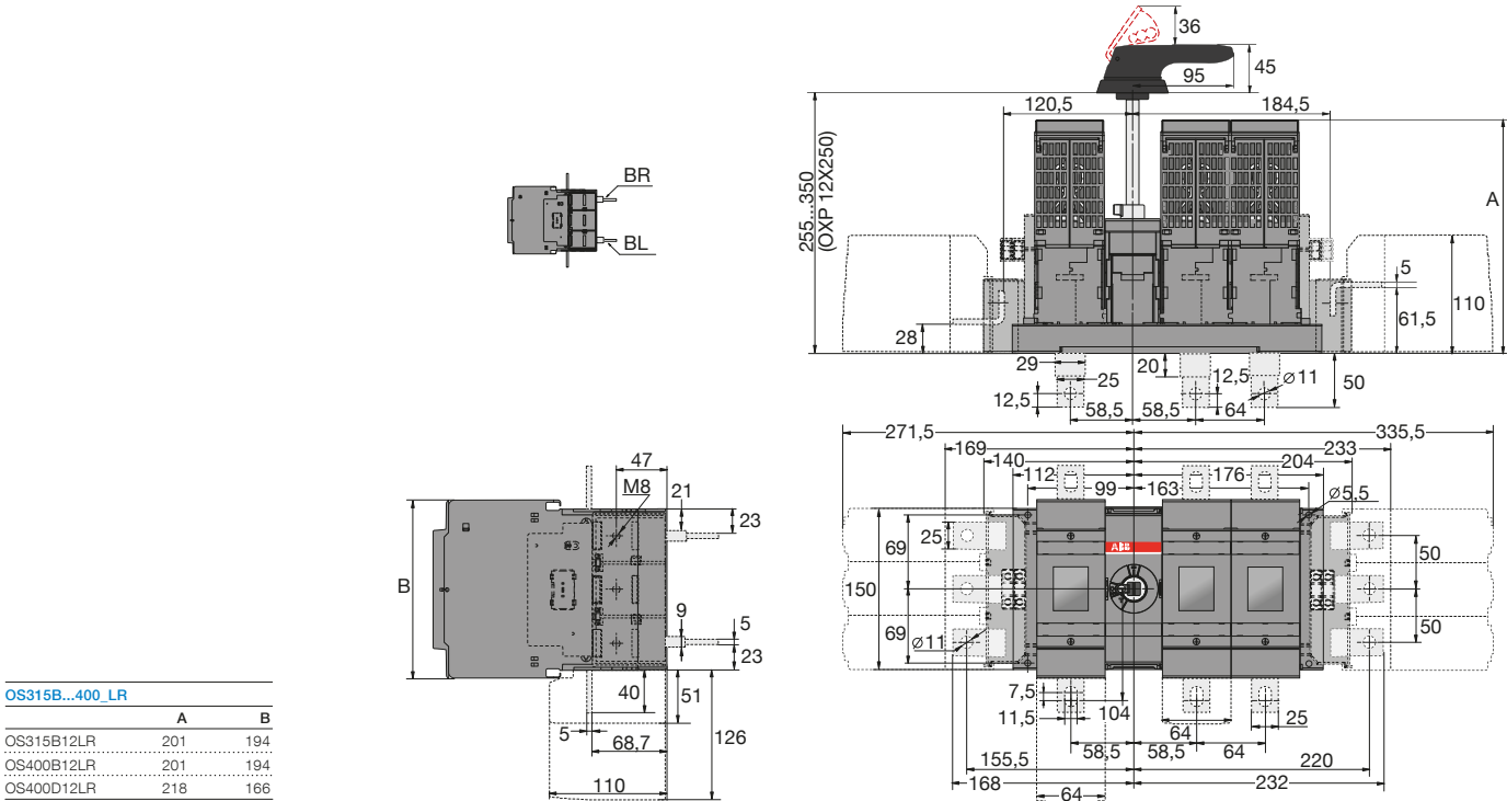
OS315B12_ and OS400_12_ (LR)
