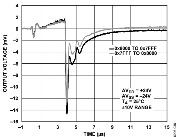
Figure 40. Digital-to-Analog Glitch
