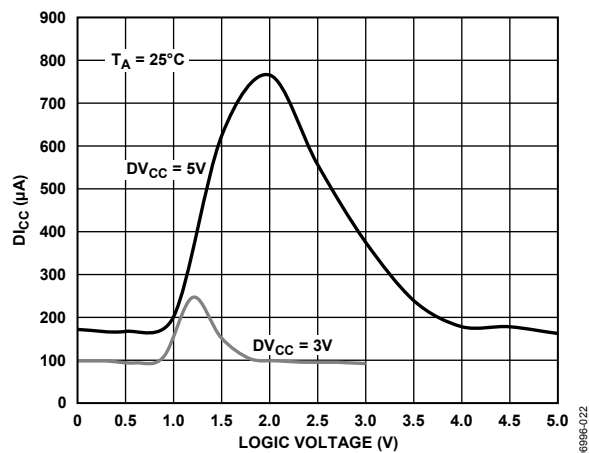
Figure 7. D_{II} vs. Logic Input Voltage
