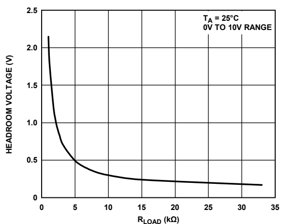
Figure 34. V_{OUT} Headroom
