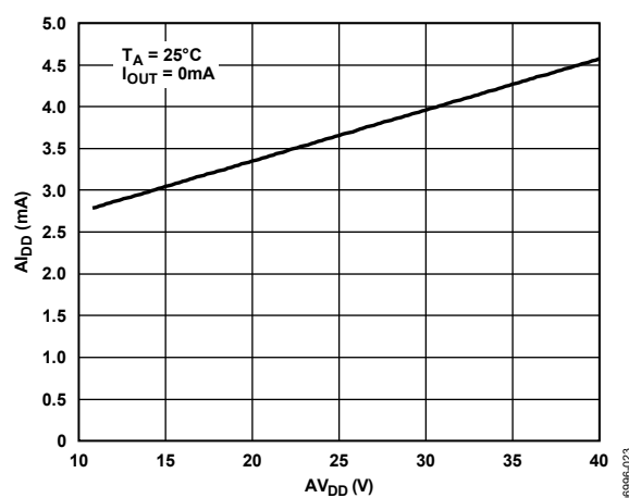
Figure 9. A_{II} vs. AV_{DD}
