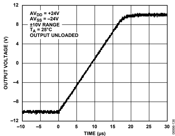
Figure 38. Full-Scale Positive Step
