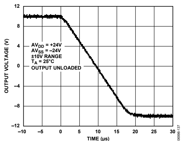
Figure 39. Full-Scale Negative Step
