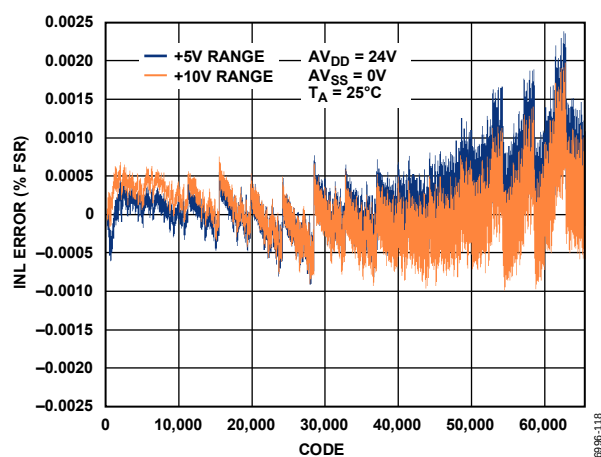
Figure 18. Integral Nonlinearity Error vs. DAC Code, Single Supply
