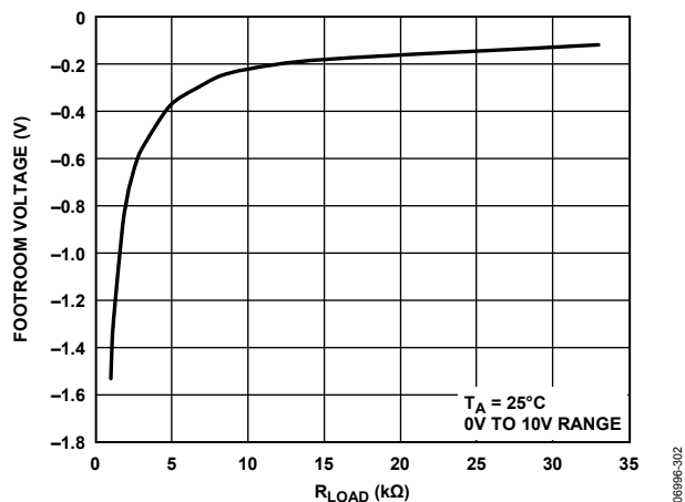
Figure 35. V_{out} Footroom
