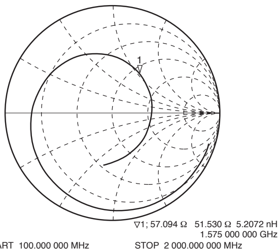
S 11 -FREQUENCY
