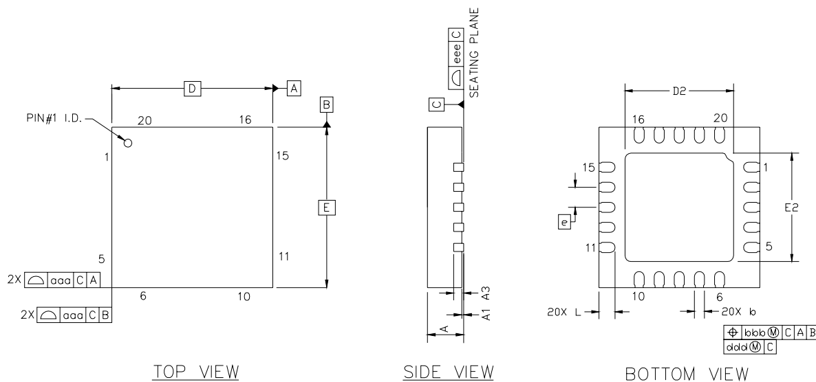
Figure 4.2. QFN-20 Package Diagram
