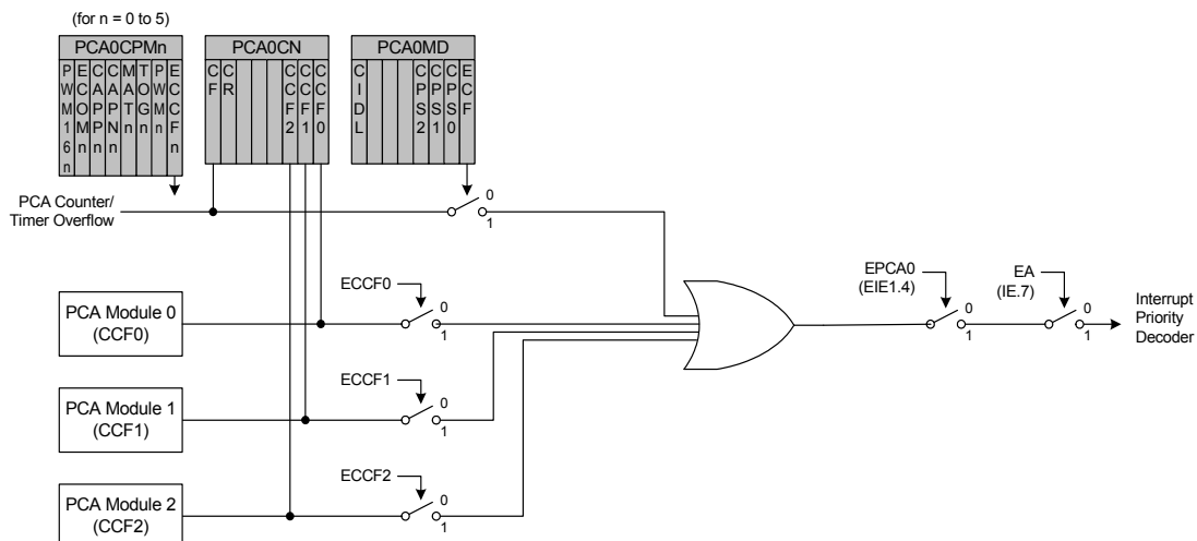
Figure 20.3. PCA Interrupt Block Diagram
