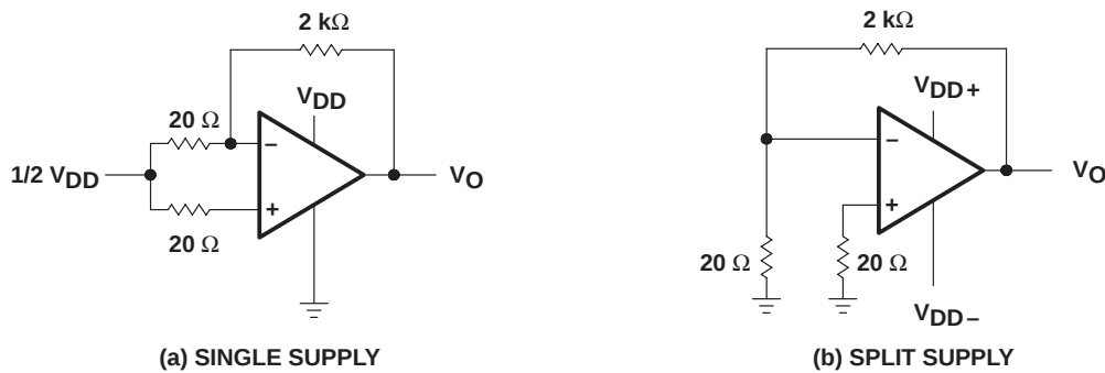
Figure 2. Noise-Test Circuit
