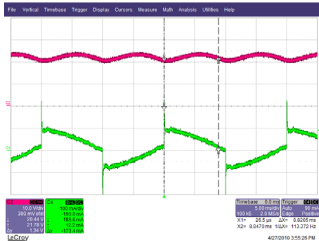
Figure 34 – 230 VAC, Full Phase. Upper: V_{OUT} , 10 V / div. Lower: I_{IN} , 0.1 A / div., 5 ms / div.
