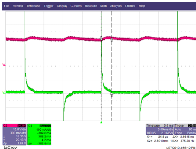
Figure 35 – 230 VAC, 49° Phase. Upper: V_{OUT} , 10 V / div. Lower: I_{IN} , 0.1 A / div., 5 ms / div.
