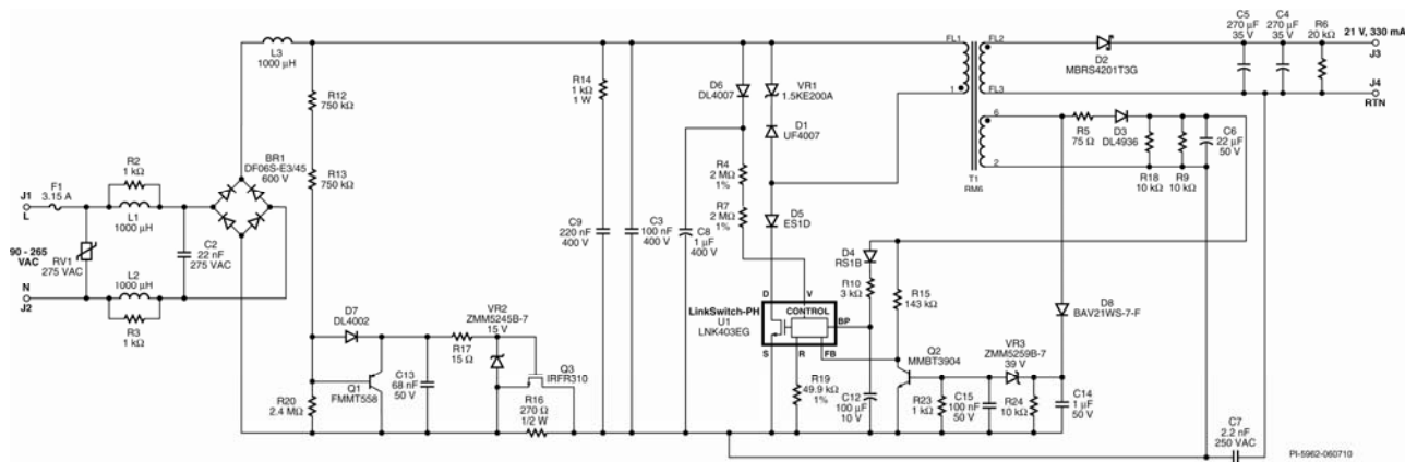
Figure 3 – Schematic.
