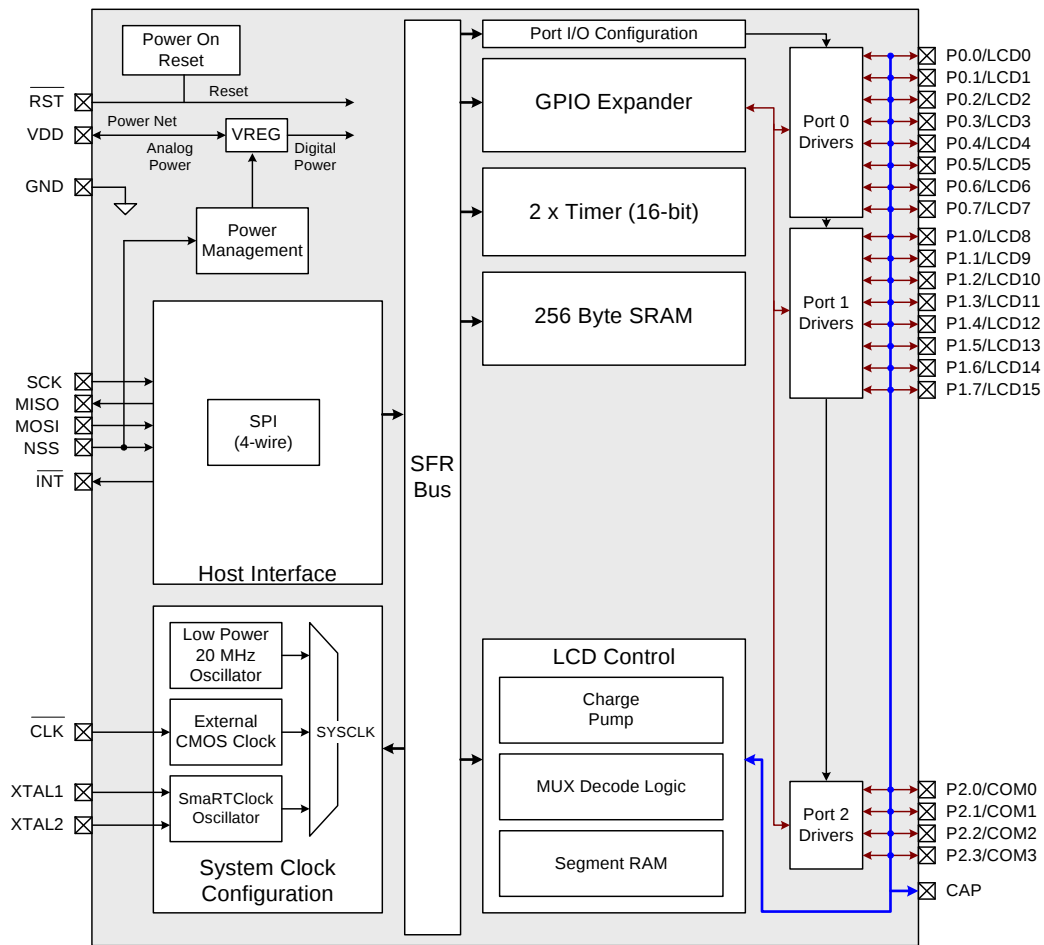
Figure 1.3. CP2402 Block Diagram
