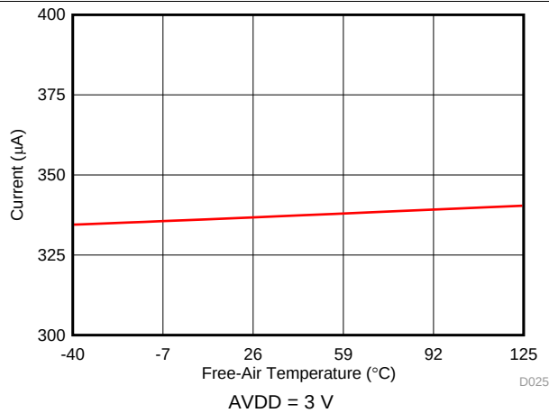
Figure 22. AVDD Supply Current vs Temperature
