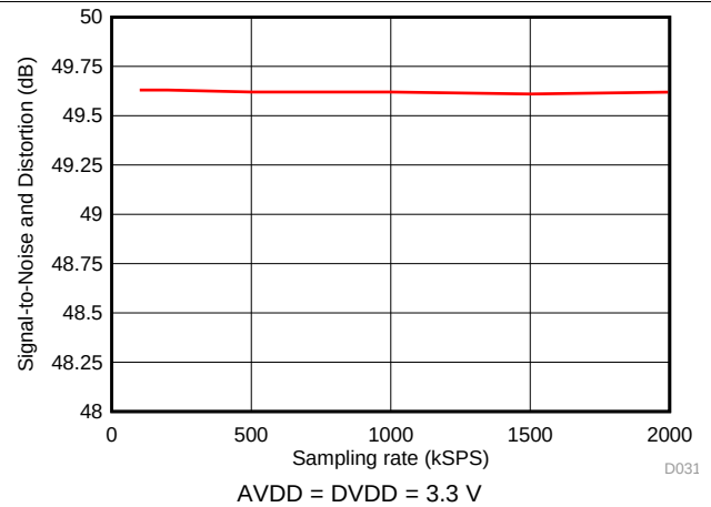
Figure 27. SINAD vs Sampling Rate
