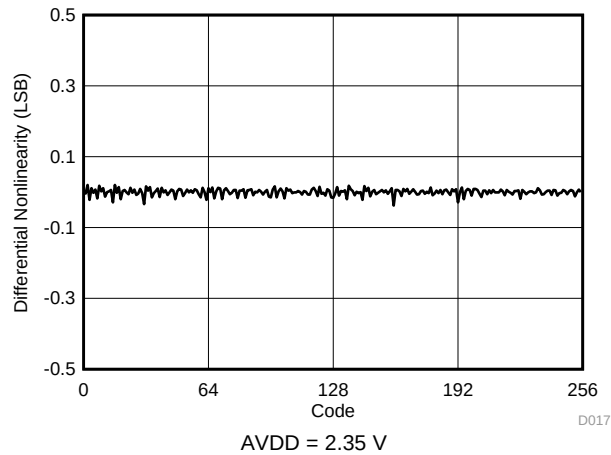
Figure 14. Typical DNL
