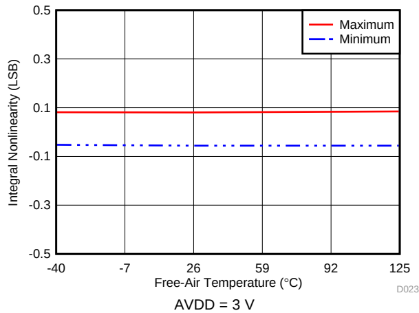
Figure 20. INL vs Temperature
