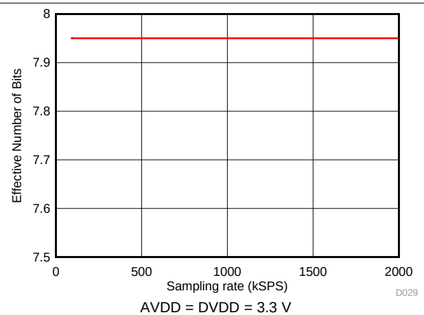
Figure 25. ENOB vs Sampling Rate
