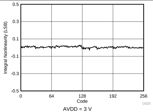
Figure 17. Typical INL
