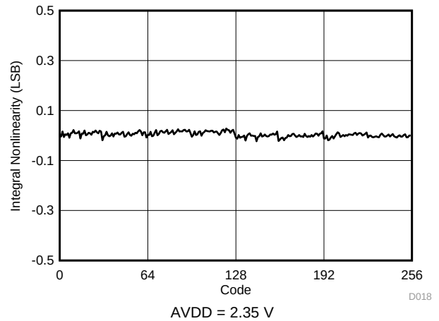
Figure 15. Typical INL
