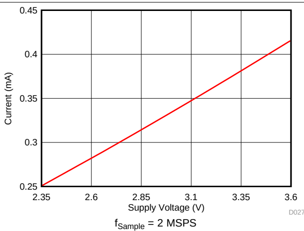
Figure 24. AVDD Supply Current vs Supply Voltage
