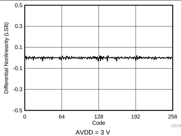
Figure 16. Typical DNL
