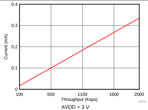
Figure 23. AVDD Supply Current vs Throughput
