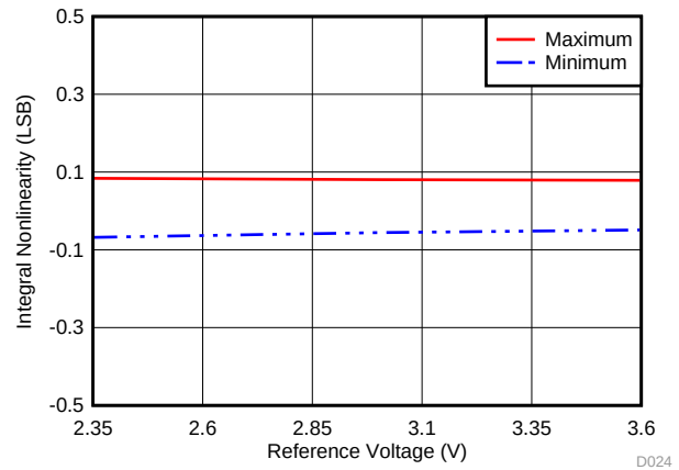
Figure 21. INL vs Reference Voltage (AVDD)
