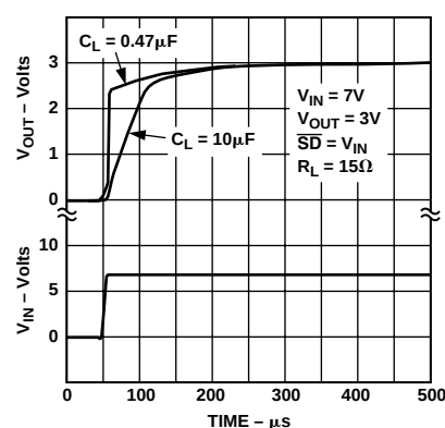
Figure 10. Power-Up Response
