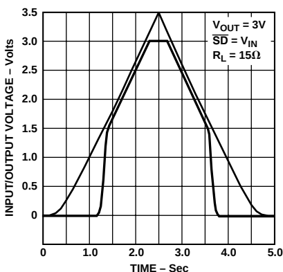
Figure 9. Power-Up/Power-Down
