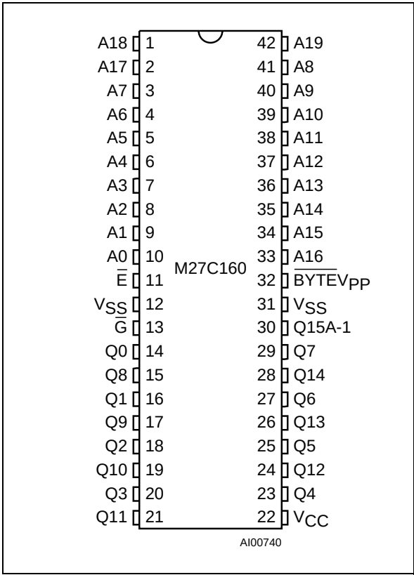
Figure 2. DIP Connections
