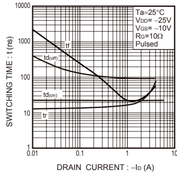
Fig.2 Switching Characteristics
