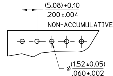
RECOMMENDED P.C. BOARD HOLE DIMENSIONS
