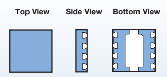
XS01 Package (1.5 x 1.5 x 0.37)
