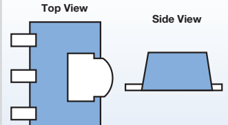
M02 Package (2.45 x 4.5 x 1.5)
