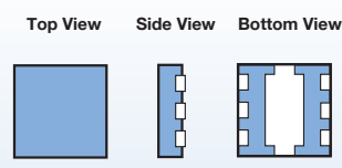
T5N / T6N Package (1.5 x 1.5 x 0.37)
