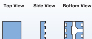
XS02 Package (1.0 x 1.0 x 0.37)
