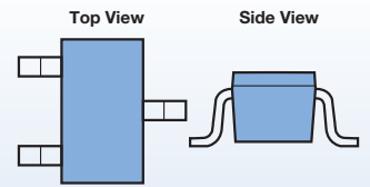
33 Package (1.5 x 2.9 x 1.4)
