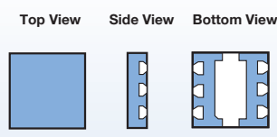
T6X Package (1.5 x 1.5 x 0.37)
