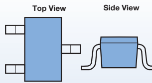
30 Package (1.25 x 2.0 x 0.9)
