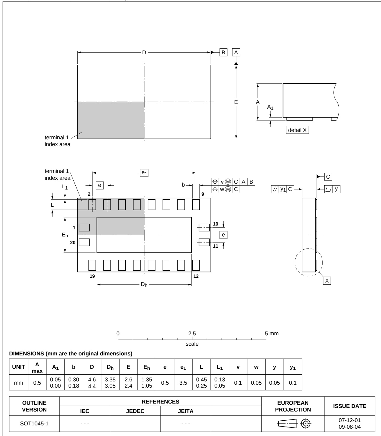
Fig 12. Package outline SOT1045-1 (DHXQFN20U)
