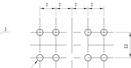
PIERCING PLAN
