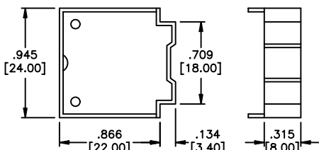
DPS8L2 Dummy housing
