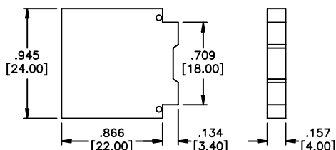
DPS8A2 Spacer
