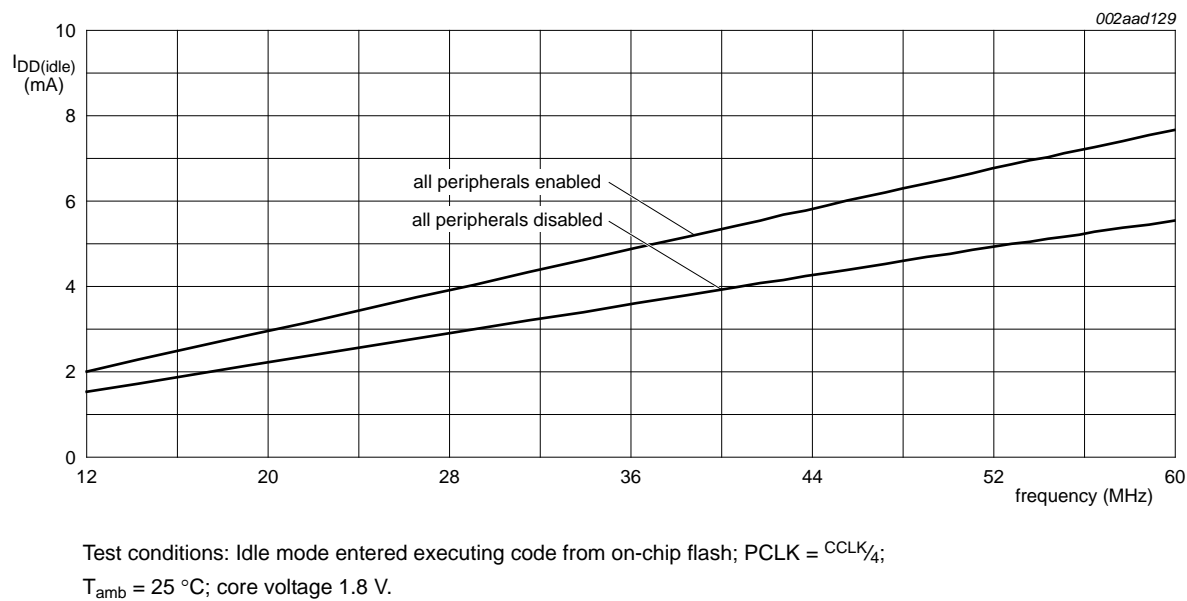
Fig 7. Typical LPC2109/01 I_{DD(idle)} measured at different frequencies
