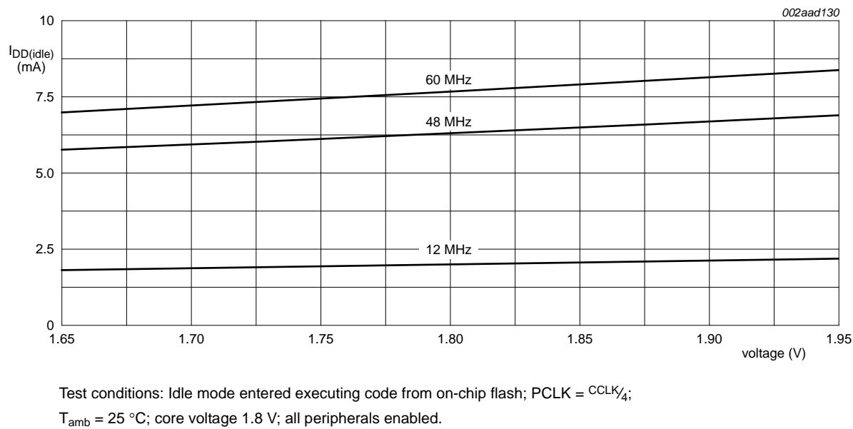
Fig 8. Typical LPC2109/01 I_{DD(idle)} measured at different voltages
