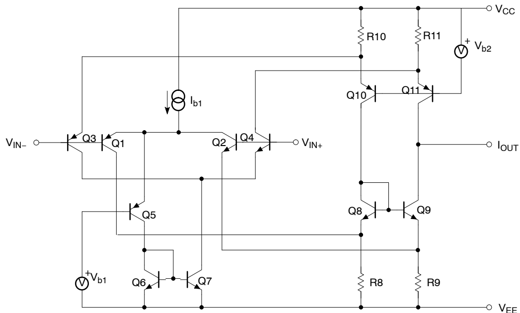
Figure 1. Input Stage
