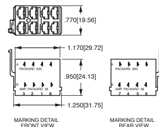
VCH CONNECTOR HOUSING
