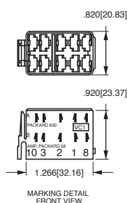
VC1 CONNECTOR HOUSING
