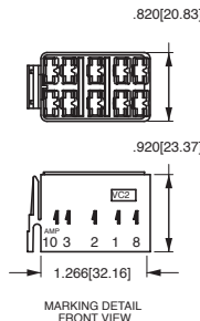
VC2 CONNECTOR HOUSING (For AMP terminals only)
