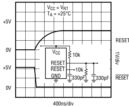
MAX707 RESET, RESET DE-ASSERTION
