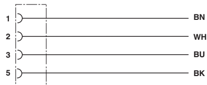
Contact assignment of 7/8" socket
