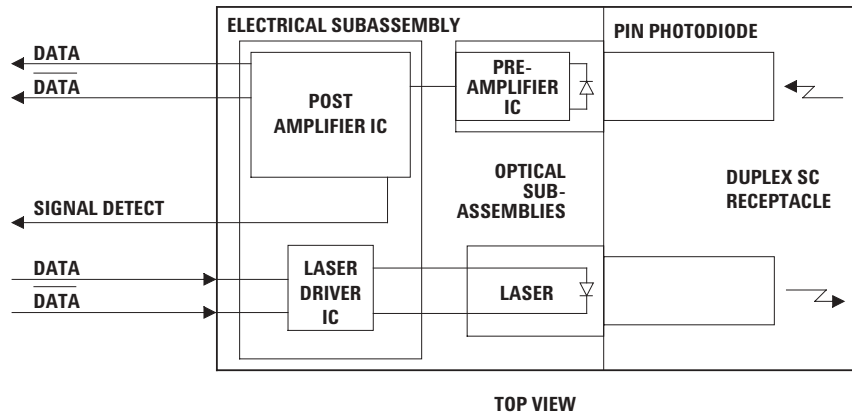
Figure 1. Block Diagram
