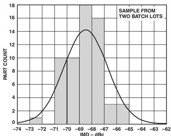
TPC 32. Distribution of \text{IMD}_3 , 70 MHz, R_L = 1\text{ k}\Omega , V_{\text{OPHI}} - V_{\text{OPLD}} = 1\text{ V p-p Composite} , V_S = 5\text{ V} , Maximum Gain
