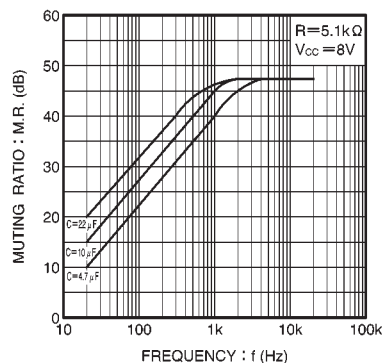
Fig. 14 Muting ratio vs. frequency
