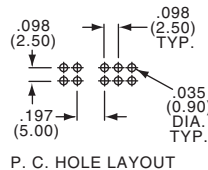
P. C. HOLE LAYOUT
