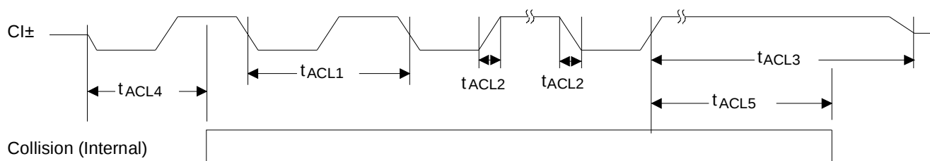
Figure 46. AUI Collision
