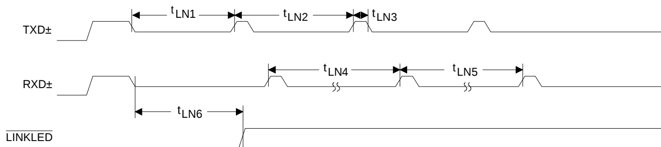
Figure 58. 10BASE-T Link Integrity
